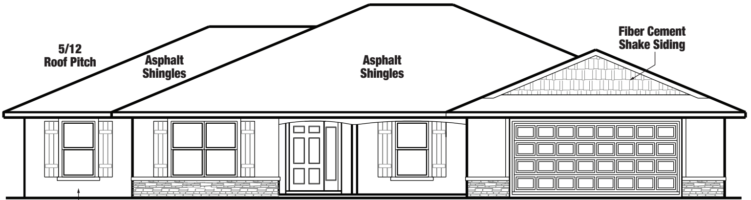
Front Elevation
